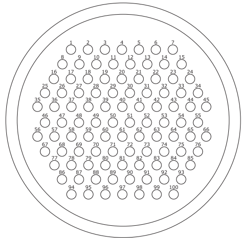
100 pin | size 40 (SVK-SHD)
