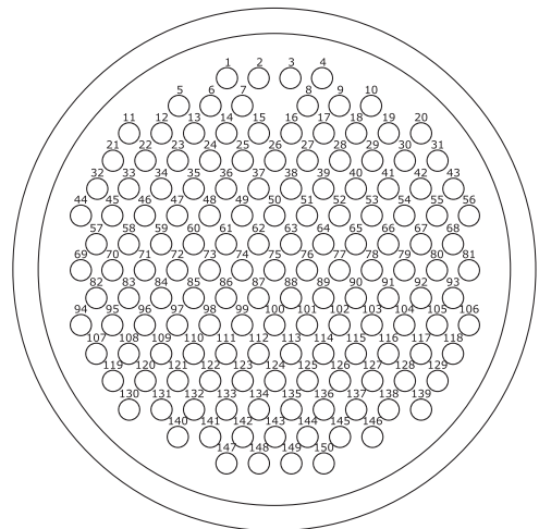
150 pin | size 40 (SVK-SHD)
