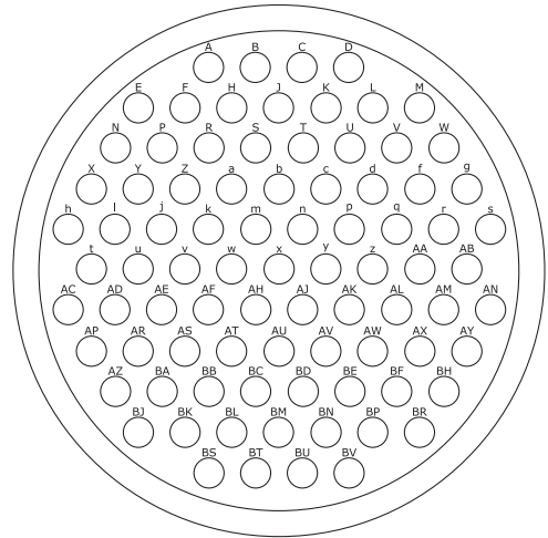
85 pin | size 40 (SVK-SHD)
