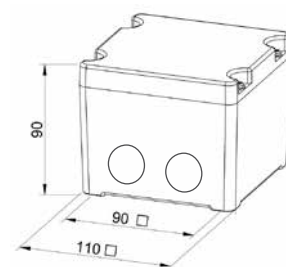
Enclosure D5 Material Die-Cast Aluminium Colour Grey (RAL 7035) Red (RAL 3020) Entries 2 x M20 Fixings 4 x M5
