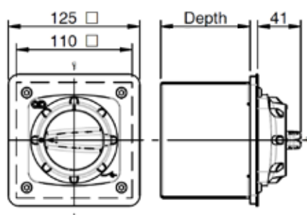
IP65 Back Box Size A
