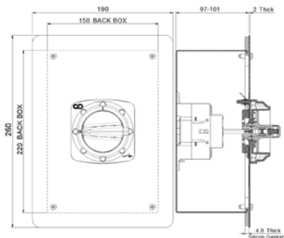
IP65 Back Box Size D
