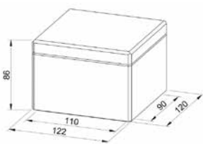
Enclosure D2 Material Polycarbonate Colour Grey (RAL 7035) Entries Plain sides Fixings 2 x M4
