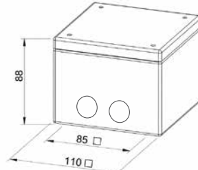
Enclosure D9 Material Stainless Steel (Grade 304) Colour Brushed Entries 2 x M20 Fixings 4 x M6
