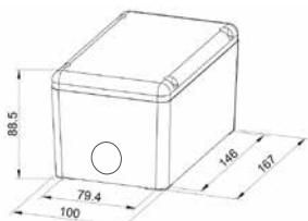
Enclosure D7 Material Die-Cast Aluminium Colour Grey (RAL 7035) Entries 1 x M20 Fixings 4 x M5
