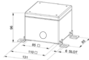
Enclosure D10 Material Stainless Steel (Grade 304) Colour Brushed Entries 1 x M20 Fixings 4 x M6
