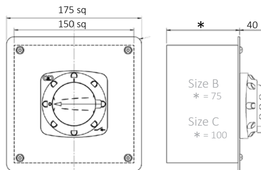
Standard Size B (* = 75) / Size C (* = 100)
