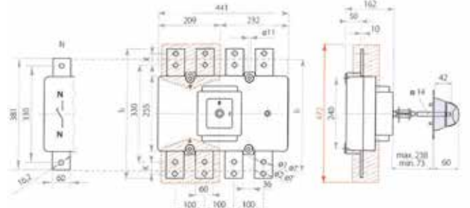
T4 Size (1600A)
