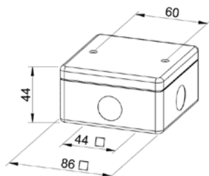
Enclosure D8 Material Steel Colour Silver Entries 5 x M20 knockouts Fixings 4 off 5 x 10 slots
