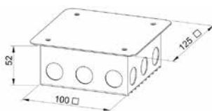
Enclosure D11 Material Fascia Plate - Stainless Steel Back Box - Galvanised Steel Colour Fascia Plate - Brushed Entries 9 x M20 knockouts Fixings 4 x M5
