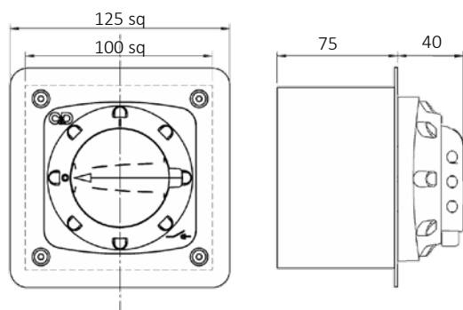
Standard Size A
