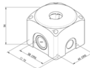
Enclosure D12 Material Polycarbonate Colour Yellow/Black Entries 2 x M20/M25/ PG13.5/PG16 2 x M16/PG11 Fixings 4xM4
