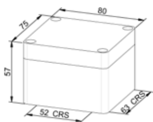
Enclosure D0 Material Die-Cast Aluminium Colour Grey (RAL 7001) Entries Plain sides Fixings 2 x M4
