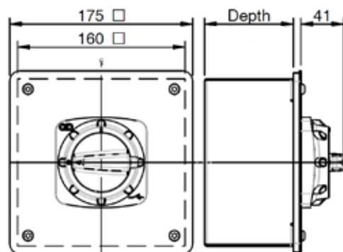
IP65 Back Box Size B / Size C
