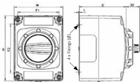
Sizes A & B
