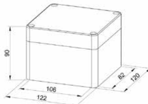
Enclosure D4 Material Glass reinforced Polyester Colour Grey (RAL 7001) Entries Plain sides Fixings 4 x M5
